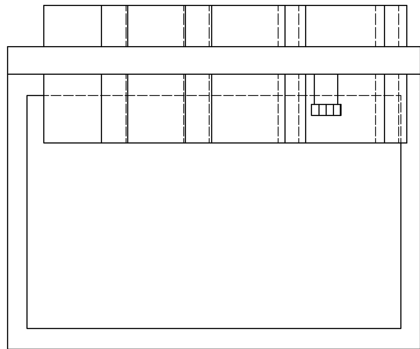
Front view
